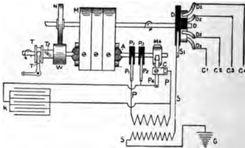
FIG. 199.—Circuit Diagram of the Eisemann High-tension Magneto. A, armature; C, primary circuit breaker; C 1 , C 2 , C 3 , C 4 , high-tension leads to cylinders; D, high-tension distributor disc; D 1 , D 2 , D 3 , D 4 , distributor wiper contacts; G, primary ground on metal of engine; K, condenser; M, permanent magnets; N, gear on distributor shaft; P, P, primary circuit of induction coil; P 1 , P 2 , wiper contacts on distributor rings; P, P, primary circuit; S, S, secondary circuit; T, bell crank for timing; T 1 , spool in which bell crank works; T 2 , slotted sleeve on driven shaft; W, gear on driven shaft.
